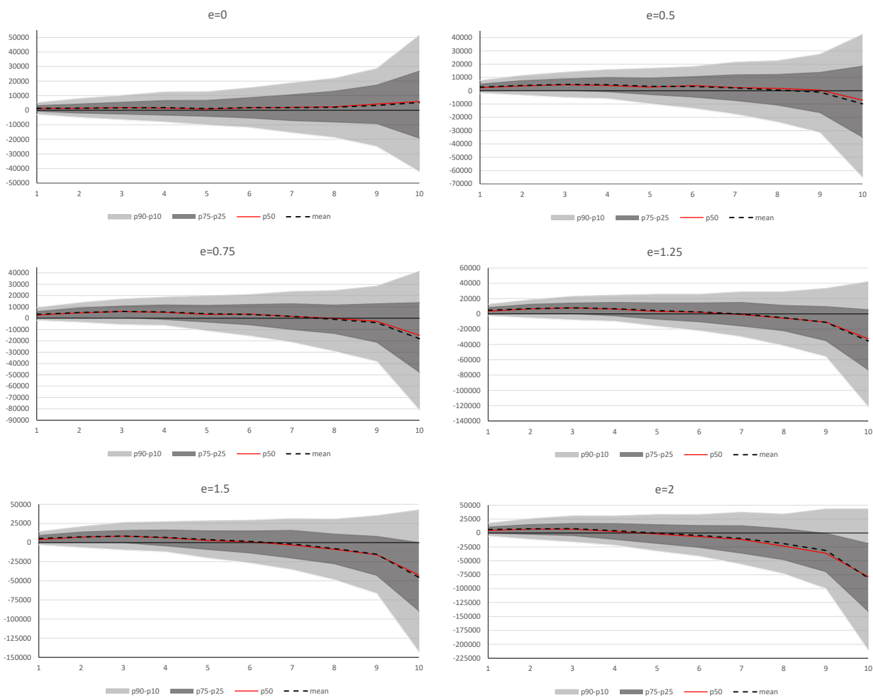
Figure D.1: Within decile quantile values of welfare changes
